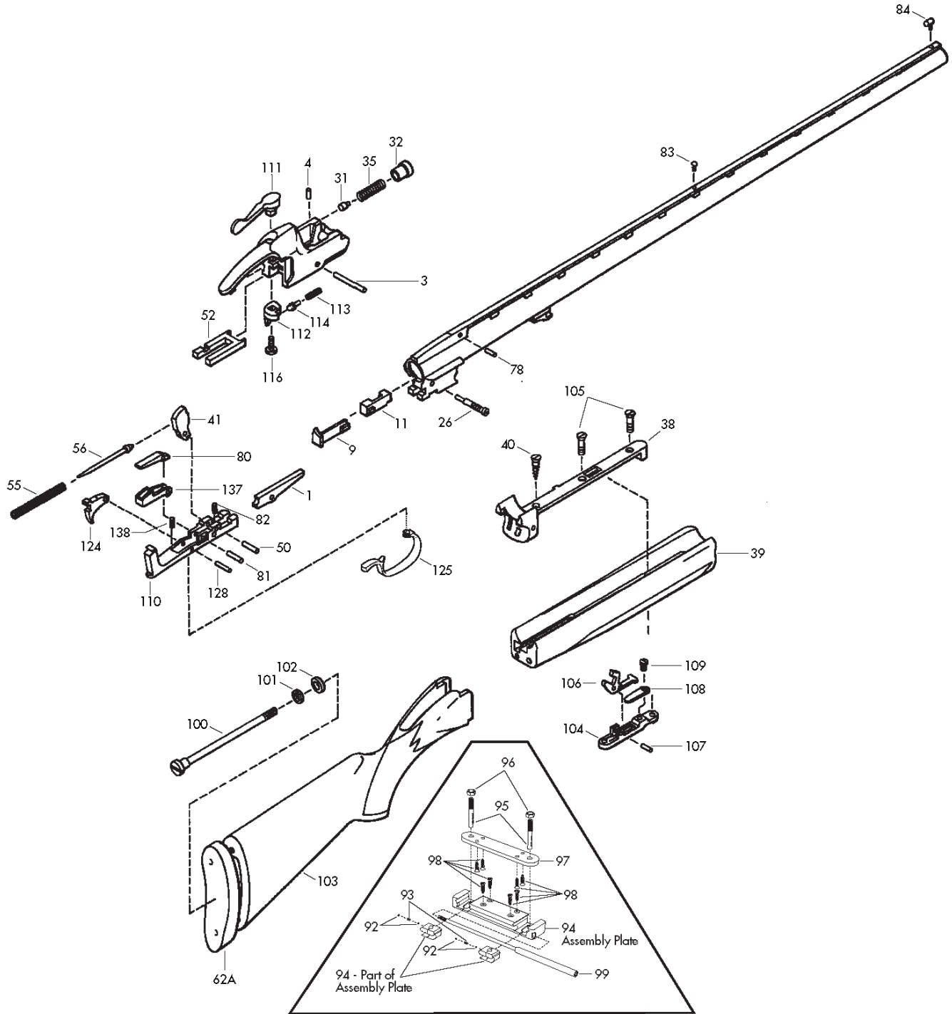
Parts for New Style Adjustable Comb Stock
